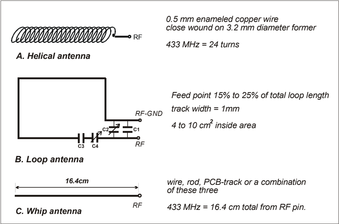
Fig.7: Antenna
