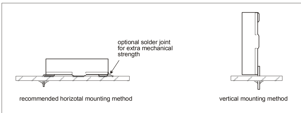
Figure 6: Module mounting options
